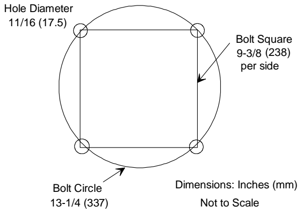
Beacon Mounting Pattern
